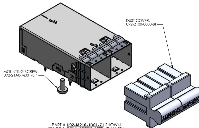
PART # U92-M216-1D01-71 SHOWN (CAGE & CONNECTOR ASSEMBLY WITH WITH SCREWS AND WITHDUST COVER SHIPPED BULK)
