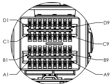
DETAIL A SCALE 6:1
