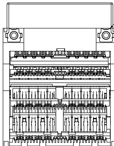
V62-CFZ01-040031T (WITH SOLDER RING)
