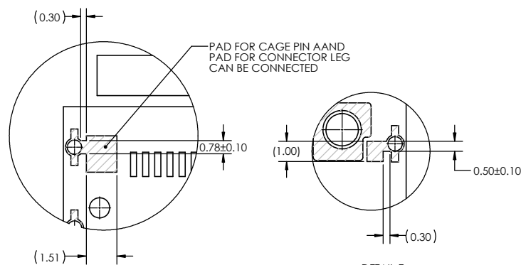
DETAIL E SCALE 8 : 1
