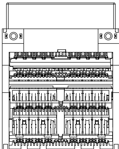
V62-CFZ01-040030T (WITHOUT SOLDER RING)
