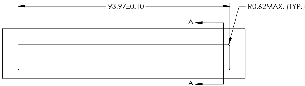
RECOMMENDED BEZEL DESIGN FOR SINGLE SIDE MOUNTING
