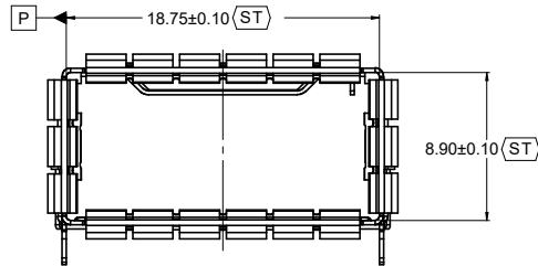
DETAIL B SCALE 20 : 1
