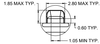
DETAIL A SCALE 5 : 1
