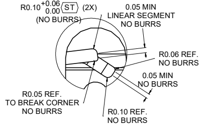
DETAIL B SCALE 20 : 1
