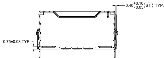
SECTION C-C SCALE 3 : 1
