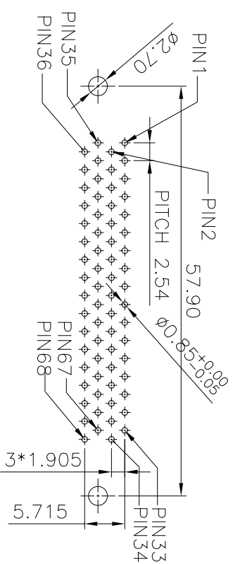
PCB LAYOUT
