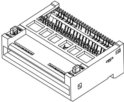
V95-AEZ01-000011T FOR SINGLE SIDE APPLICATION
